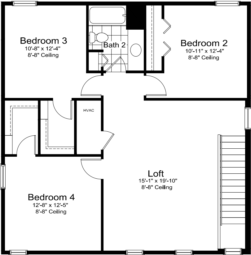
Upper Floor ALL ELEVATIONS
